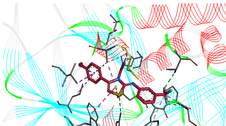
Figure 1: Super position of binding of compound 3h to the acceptor site of gamma butyrobetaine hydroxylase
