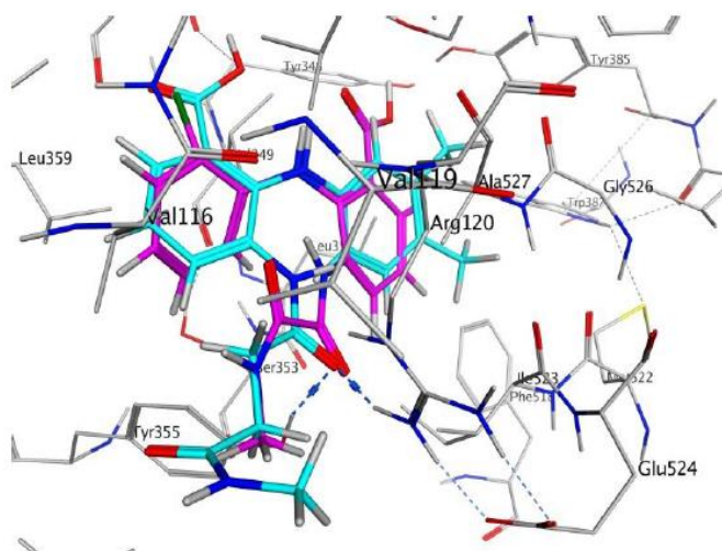
Figure 5: The superposition of the molecules of compounds 8 (lilac) and 14 (blue) in the active center of COX-
