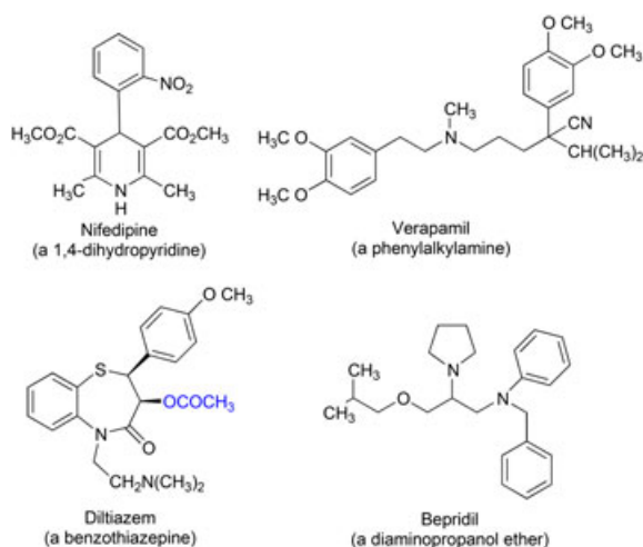
Figure 2. Main representatives of chemical classes of calcium channel blockers. [Color figure can be viewed at wileyonlinelibrary.com]
