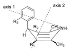
Figure 4. 1,4-DHPs general structure showing the orientation of affinity axis (axis 1) and chirality-activity axis (axis 2) on the boat conformation.
