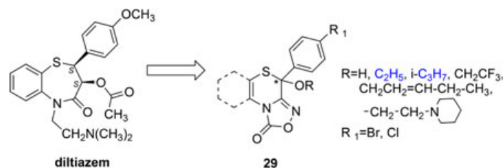
Figure 13. Discovery of new dual acting oxadiazolothiazinone derivatives. [Color figure can be viewed at wileyonlinelibrary.com ]
