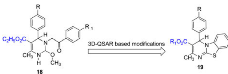
Figure 8. Development of pyrimidobenzothiazole-3-carboxylate derivatives. [Color figure can be viewed at wileyonlinelibrary.com]
