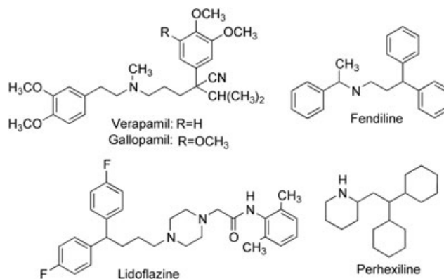
Figure 12. Phenylalkylamine calcium channel blockers.
