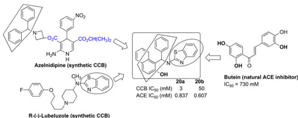
Figure 9. Design strategy for 2-(diarylalkyl)aminobenzothiazoles synthesis. [Color figure can be viewed at wileyonlinelibrary.com]
