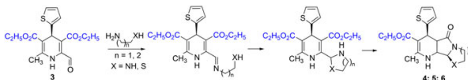
Figure 7. Synthesis of novel chiral 1,4-dihydropyridinyl Schiff-base and their further cyclization. [Color figure can be viewed at wileyonlinelibrary.com]
