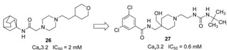
Figure 11. Design of novel T-type calcium channel inhibitors.
