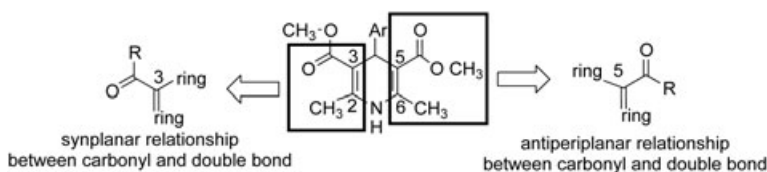
Figure 6. Conformation of the C3 and C5 esters of nifedipine (Ar = 2-nitrophenyl).
