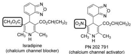
Figure 5. Structures of isradipine and its analogous 3-nitro derivative.
