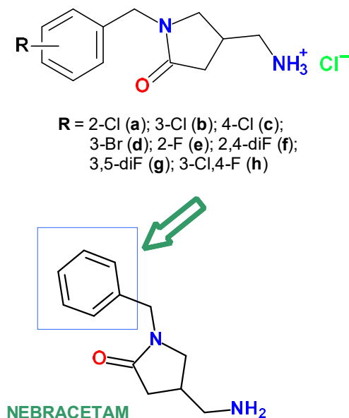
Fig. 1. A planned modification of the basic 4-(aminomethyl)-1-benzylpyrrolidine-2-one
