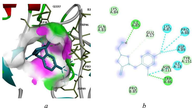
Fig. 6. Superposition of molecule 8f (R-isomer) at the allosteric site of the agonist-binding domain (ABD) of the nAChR receptor (a); diagram of intermolecular interactions (b)
