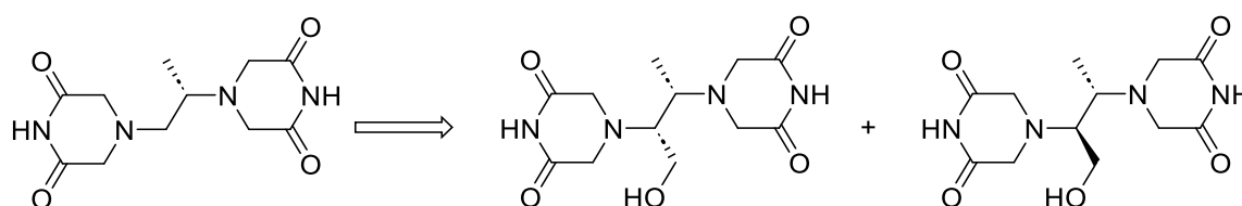
Figure 1: Scheme 1: DEX, and methylhydroxy-DEX
